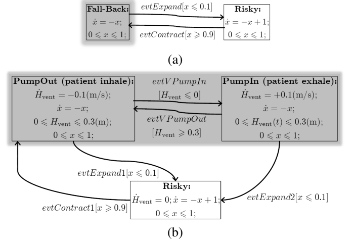
Fig. 6. Atomic Elaboration Example (compare the shaded areas in (a) and (b)). (a) Hybrid Automaton A , which has one data state variable x ; the shaded location is to be elaborated. (b) Hybrid Automaton A'' , which is the atomic elaboration of A (see (a)) at location “Fall-Back” with simple hybrid automaton A'_{\text{vent}} (see Fig. 2); note there is no edge from “Risky” to “PumpIn” because “PumpIn” is not an initial location of A'_{\text{vent}} .
