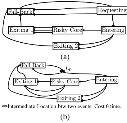
Fig. 5. (a) Sketch of Hybrid Automaton A_{\text{initzr}} , the Design Pattern for Initializer; (b) Sketch of Hybrid Automaton A_{\text{ptcpnt},i} , the Design Pattern for the i th Participant.
