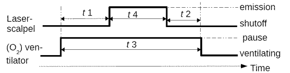
Fig. 1. Proper-Temporal-Embedding Example
