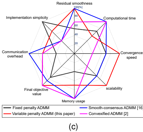
Fig. 6. Performance comparisons between different ADMM variants. (a) Weighted cost over 24 hours. (b) Convergence trends over 100 iterations. (c) Multi-metric evaluation of ADMM variants
