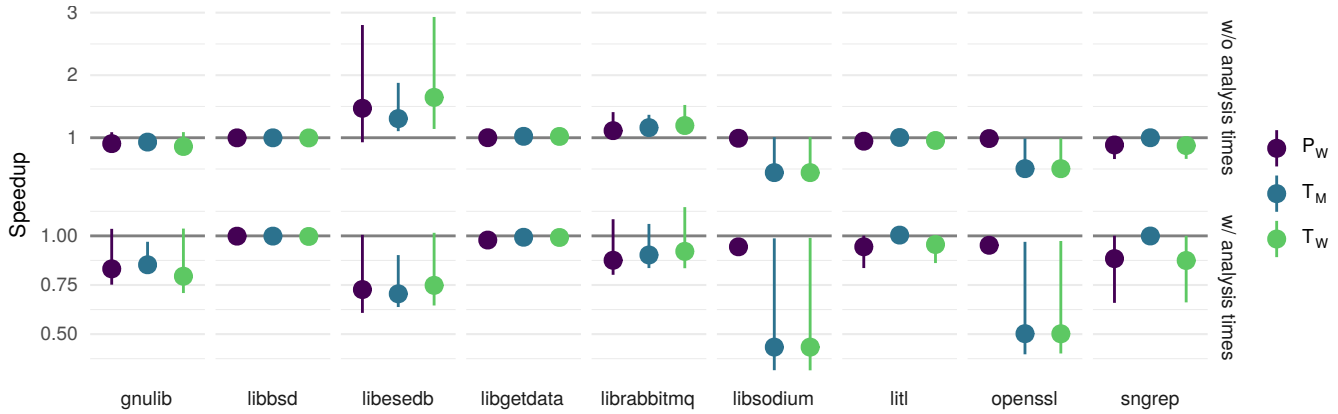
Figure 7: Geometric mean speedups relative to P_M at different degrees of parallelism. Lines indicate minimum/maximum speedups. Speedups without analysis times are based exclusively on execution times, while speedups with analysis times include the file dependency analysis for P_M and both file and global dependency analysis for the other modes.
