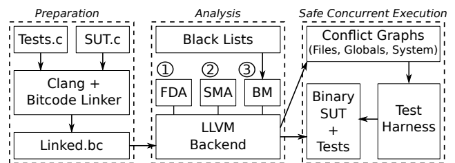
Figure 4: For our analyses, the tests and the SUT have to be compiled to bitcode and linked. After running our analyses ① – ③, which are implemented as LLVM compiler passes, we obtain information on potential test conflicts. Our test harness leverages these to derive safe parallel test schedules.
